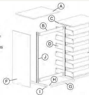
Closed-type library shelving - component anatomy
